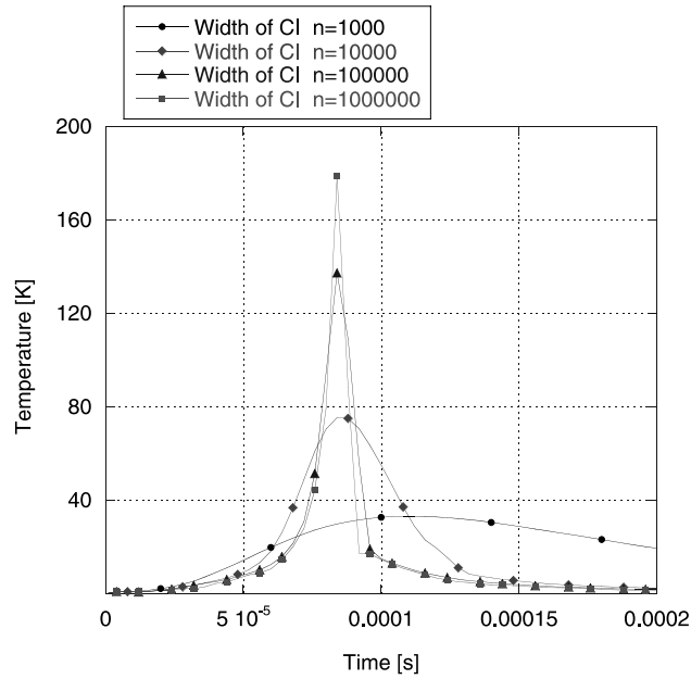
Fig. 4. Width of confidence intervals for temperature as a function of time, for different particle numbers.
