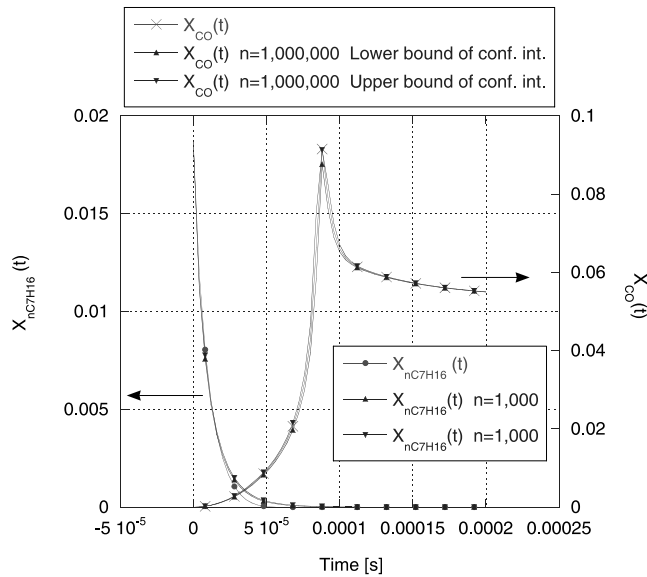
Fig. 5. Heptane and carbon monoxide need different particle numbers to have small errors.
