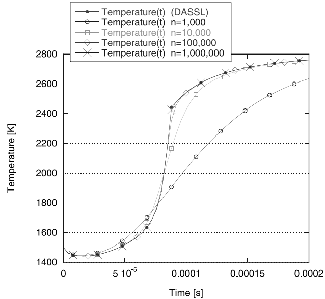
Fig. 2. Time evolution of temperature for different particle numbers. The product of particle number and repetition is constant at n \times L = 1.0 \times 10^7 .
