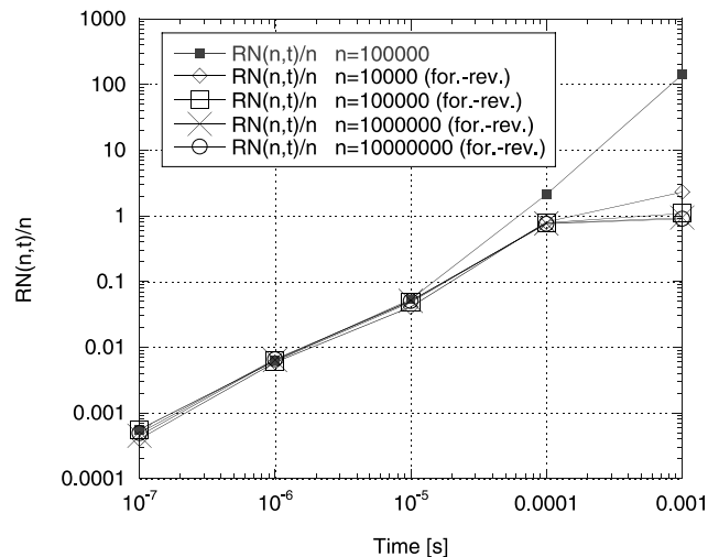
Fig. 6. Normalized reaction numbers for the direct simulation and the improved algorithm.
