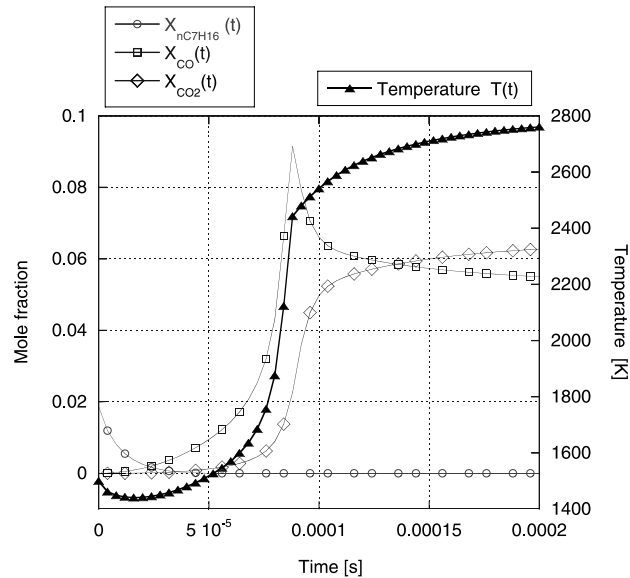
Fig. 1. Time evolution of the species' mole fractions and temperature.
