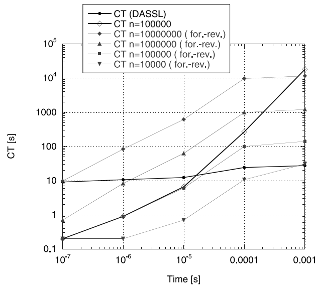
Fig. 8. Computational time as function of simulation time, for different solution methods.
