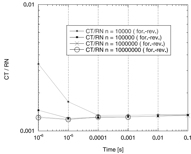
Fig. 7. Computational time divided by reaction number.
