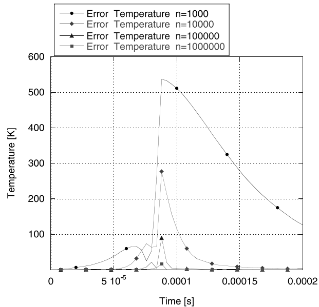
Fig. 3. Error in temperature as a function of time, for different particle numbers.
